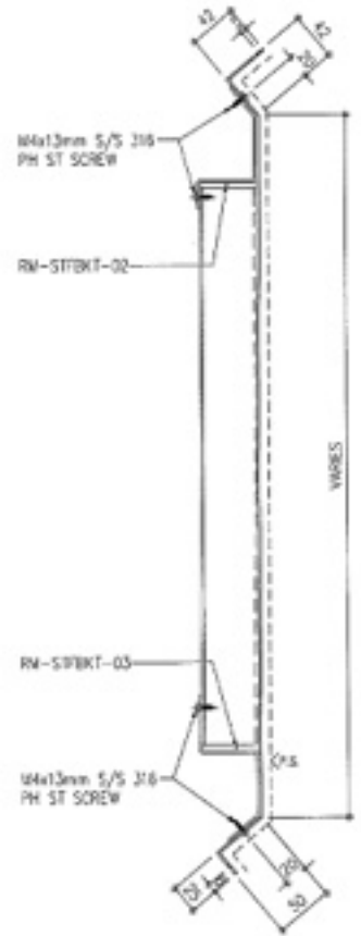
SECTION C-C
